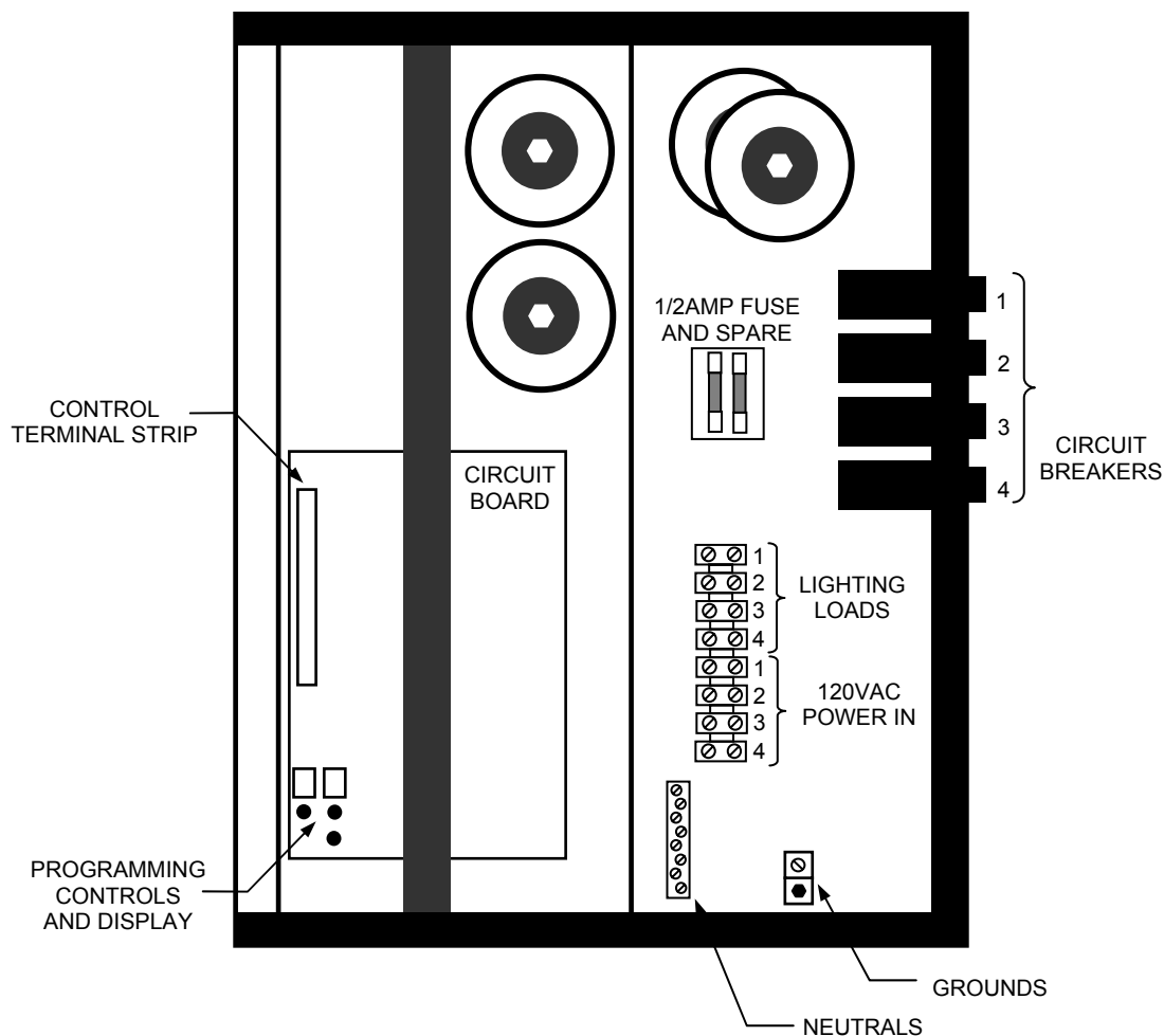
AT-402 FRONT VIEW (Cover Removed)
